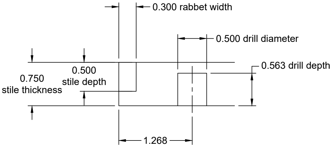
TYPICAL DETAIL
